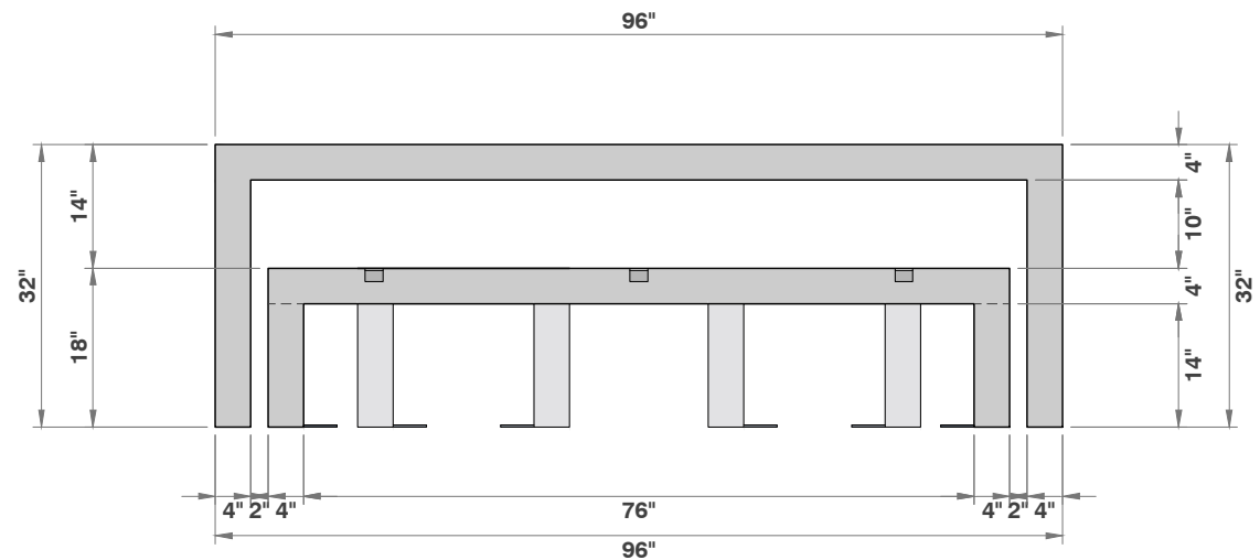
ELEVATION 1/2" = 1'
