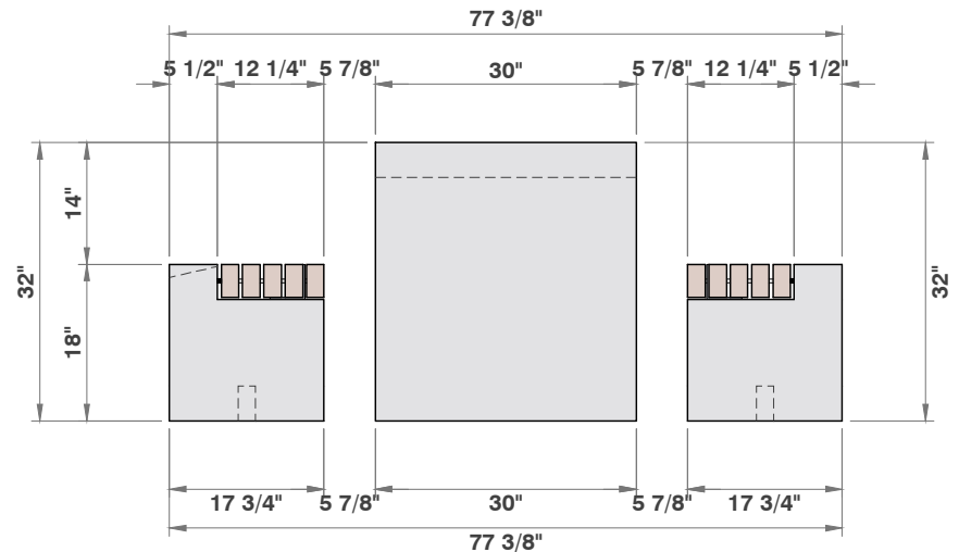
END VIEW 1/2" = 1'
