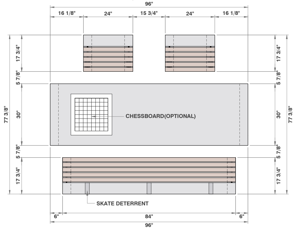
TOP VIEW 1/2" = 1'
